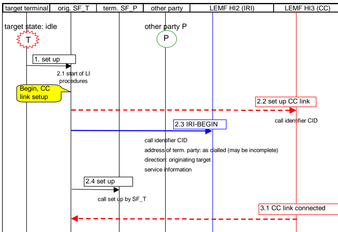
Figure E.1: Start of call originating from target
