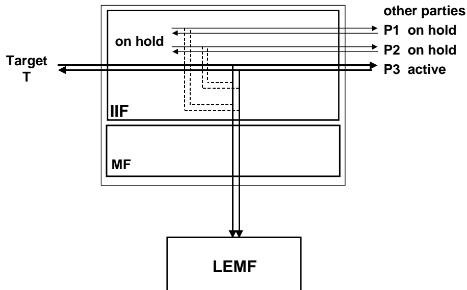
Figure 7: CC link option B (example for call hold supplementary service)
